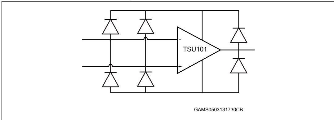
Figure 41. ESD structure
