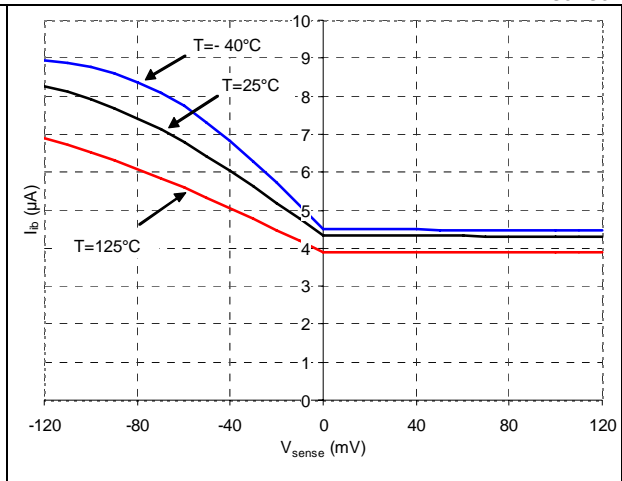
Figure 5. V_m pin input bias current vs. V_{sense}
