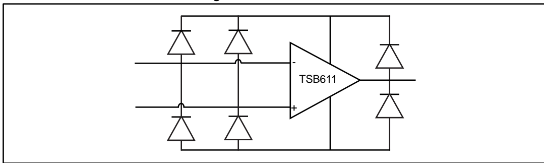
Figure 35: ESD structure
