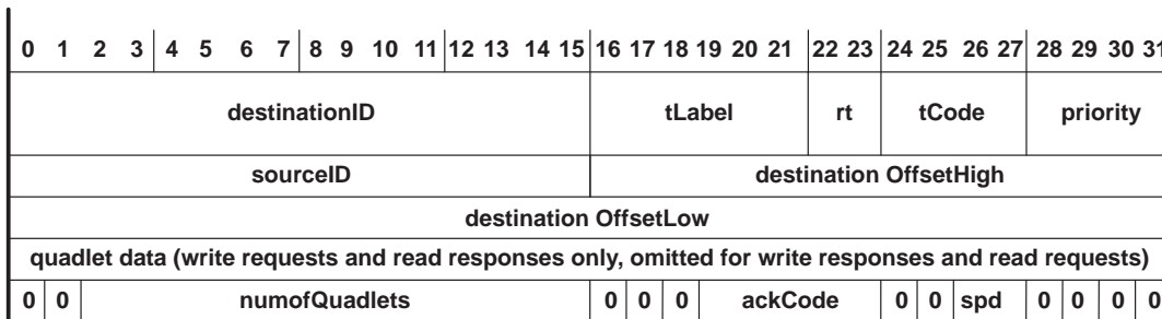
Figure 7-4. Data-Mover Quadlet-Receive Format
