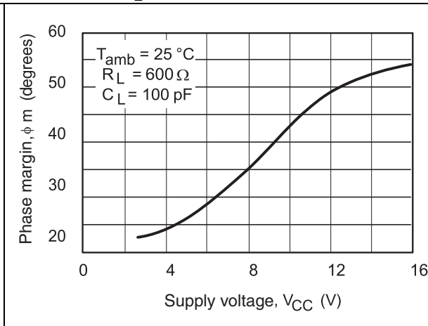
Figure 13. Phase margin vs. supply voltage ( R_L = 600\text{ }\Omega )
