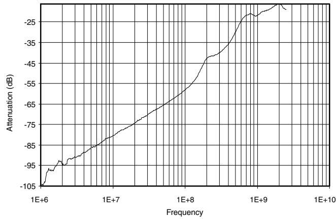
Figure 3. Crosstalk vs Frequency
