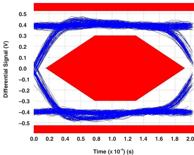
Figure 8. Eye Pattern: 480-Mbps USB Signal With Switch 2D Path
