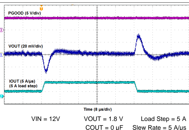
Figure 15. Transient Response
