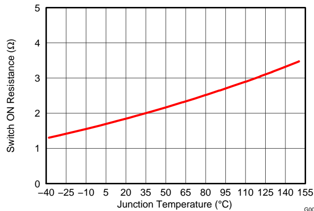
Figure 5. Switch On-Resistance ( R_{DS(on)} ) vs. Temperature
