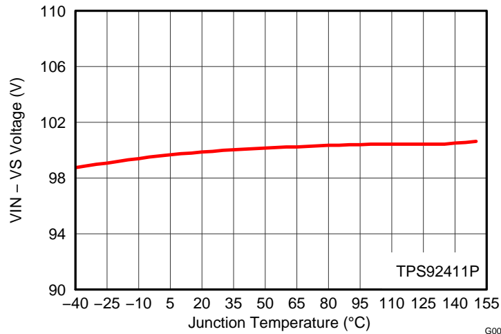
Figure 7. (VIN - VS) Overvoltage Threshold vs. Temperature
