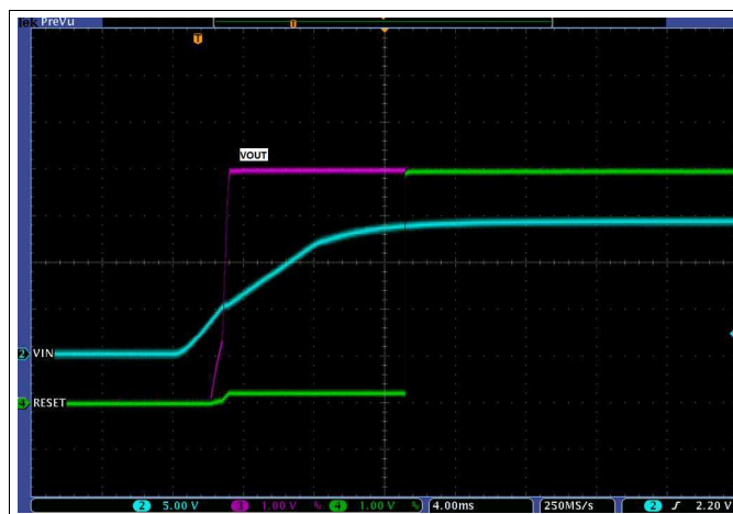
Figure 23. TPS7B6750-Q1 Power-Up Waveform
