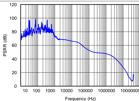
Figure 12. Power-Supply Rejection Ratio vs Frequency ( V_I = 14 V, C_O = 47 \mu F, I_L = 25 mA)
