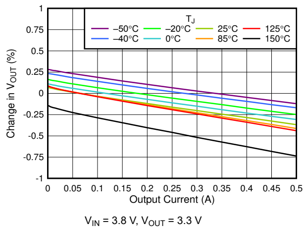
Figure 6-16. 3.3-V Load Regulation vs I_{OUT}
