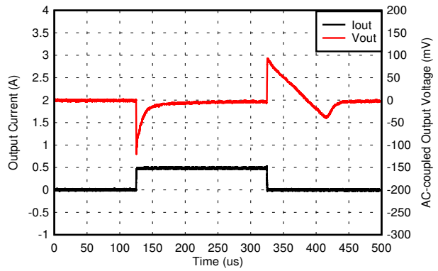
V_{IN} = 3.8\text{ V} , V_{OUT} = 3.3\text{ V} , I_{OUT} slew rate = 1\text{ A}/\mu\text{s}
