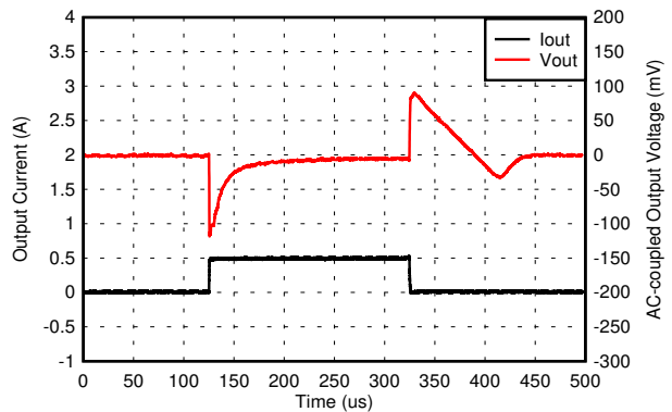
V_{IN} = 5.5\text{ V} , V_{OUT} = 5\text{ V} , I_{OUT} slew rate = 1\text{ A}/\mu\text{s}
