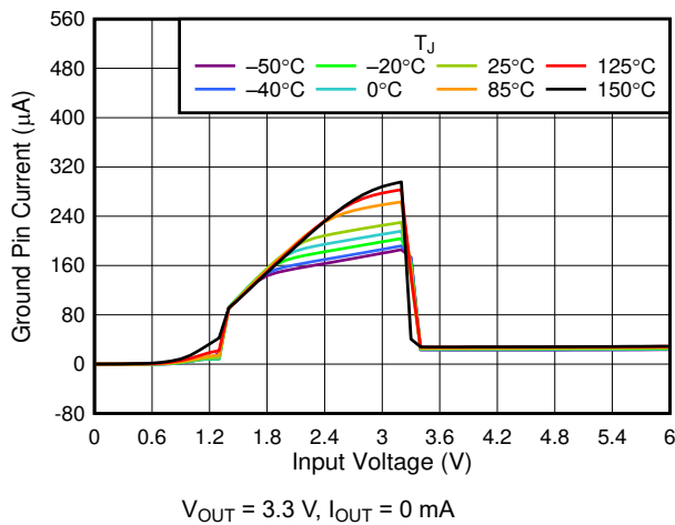
Figure 6-15. I_Q vs V_{IN}
