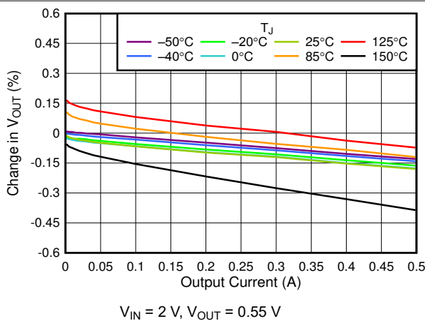
Figure 6-17. 0.55-V Load Regulation vs I_{OUT}
