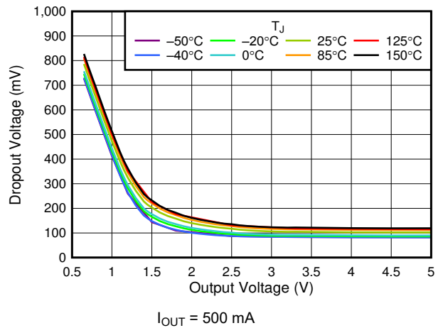
Figure 6-12. V_{DO} vs V_{OUT}
