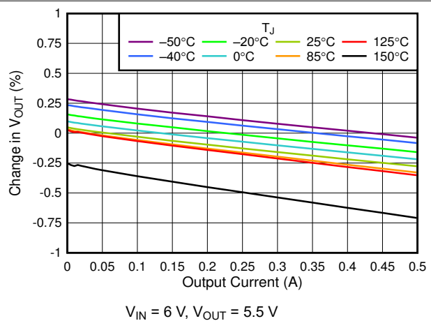
Figure 6-18. 5.5-V Load Regulation vs I_{OUT}
