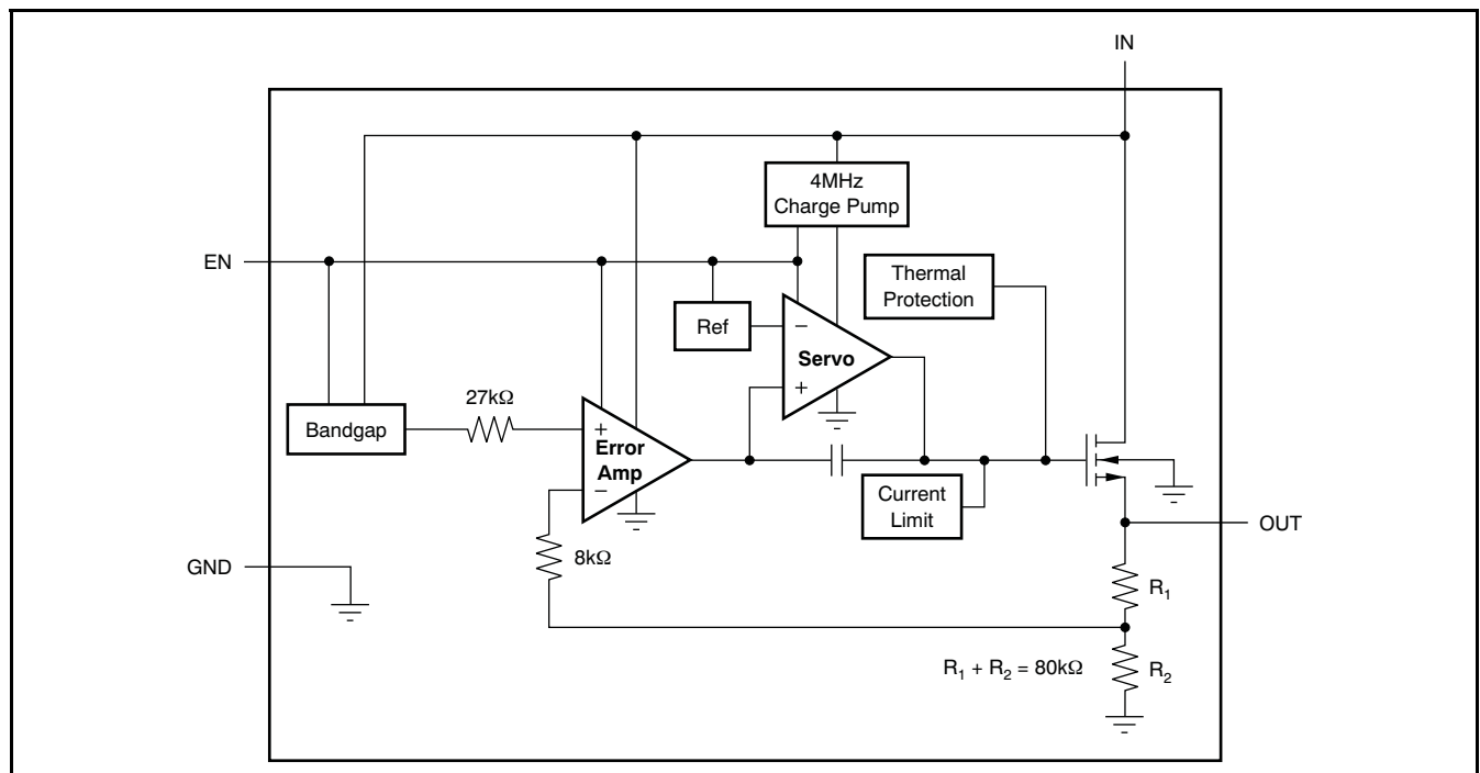
Figure 2. Fixed-Voltage Version
