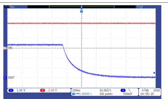
Figure 33. TPS73601 Shutdown
