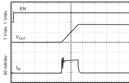
V IN = 2.1 V, V OUT = 1.8 V, I OUT = 100 μA
