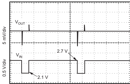
Slew rate = 1 V/μs, I OUT = 200 μA
