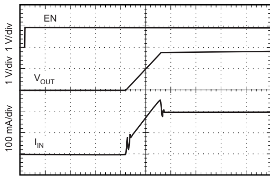
V IN = 2.1 V, V OUT = 1.8 V, I OUT = 200 mA
