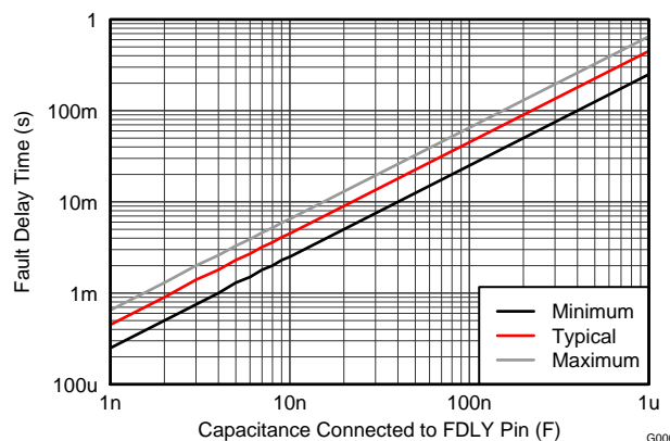
Figure 15. Adjustable Fault Delay Time
