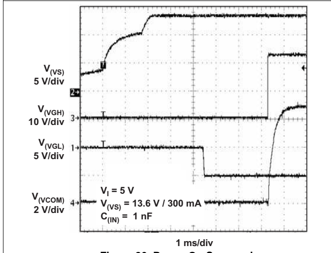
Figure 26. Power-On Sequencing
