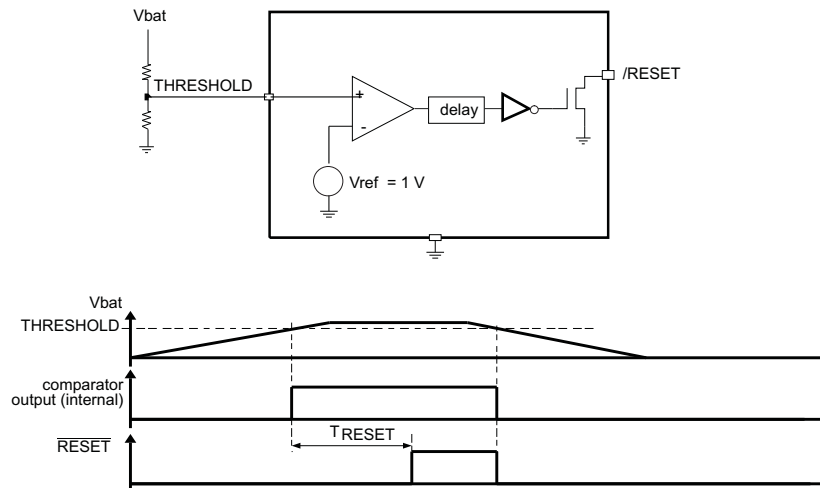
Figure 32. \overline{\text{Reset}} Timing
