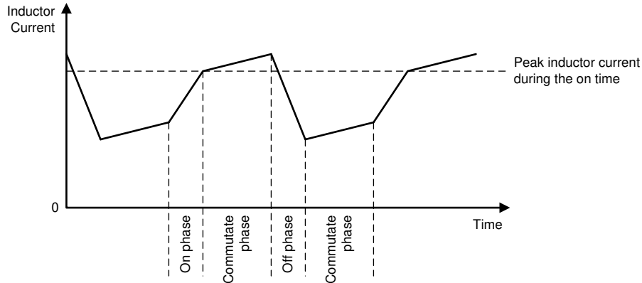
Figure 7. Peak Current Control – Buck-Boost Operation with V_1 > V_O
