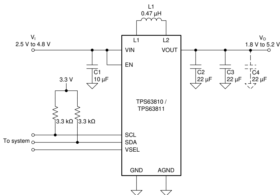
Figure 29. Typical Application Schematic
