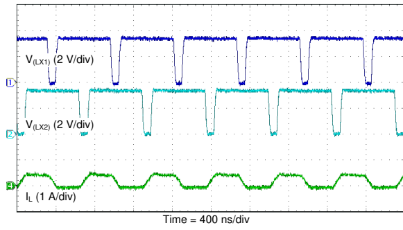
Figure 36. PFM Switching Waveforms (Boost Operation)
