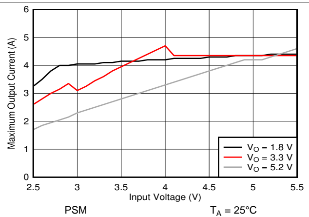
Figure 53. Maximum Output Current versus Input Voltage
