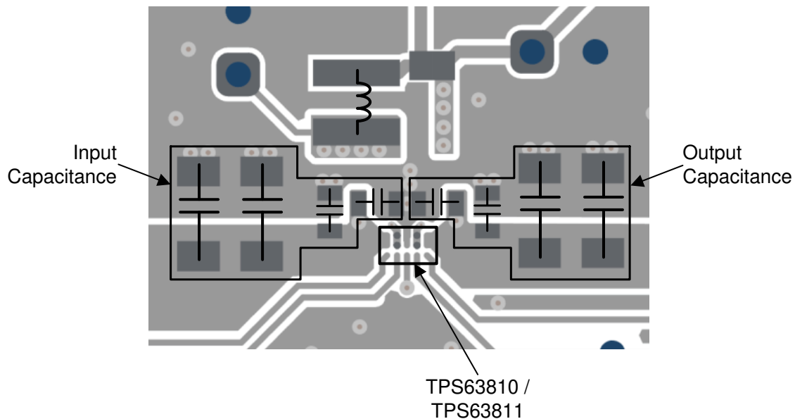
Figure 54. Recommended PCB Layout for the TPS63810 Device
