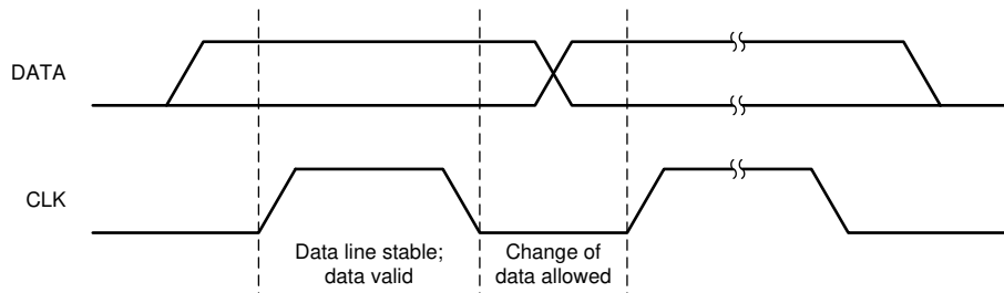
Figure 19. Bit Transfer on the Serial Interface
