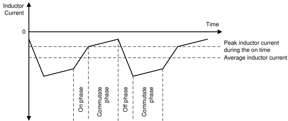
Figure 10. Reverse Peak Current Control – Buck-Boost Operation, with V_1 > V_O
