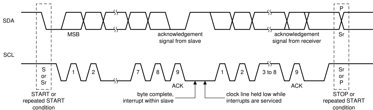
Figure 21. Bus Protocol
