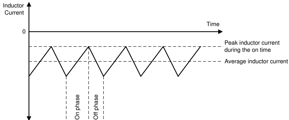
Figure 9. Reverse Peak Current Control – Buck and Boost Operation
