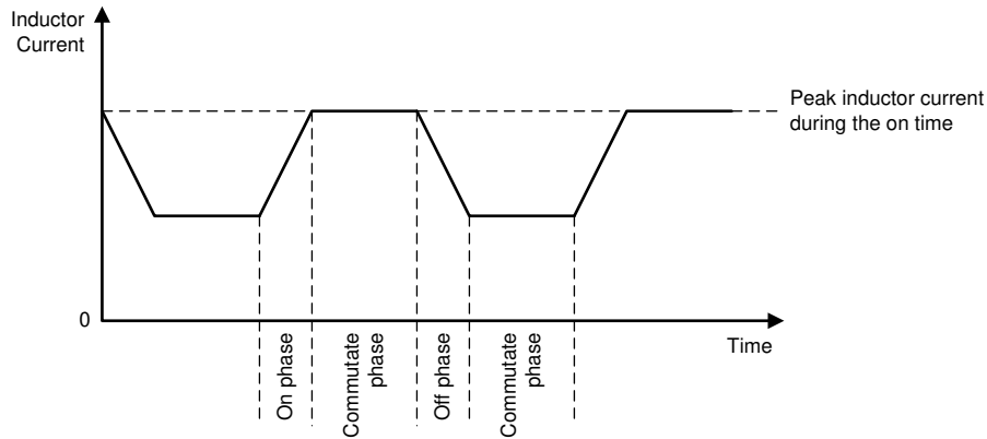
Figure 8. Peak Current Control – Buck-Boost Operation with V_1 = V_O
