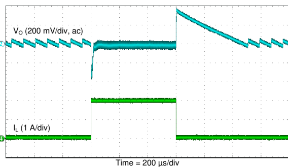
Figure 42. Load Transient Response (Buck)
