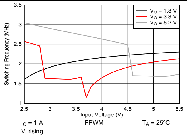
Figure 51. Switching Frequency versus Input Voltage
