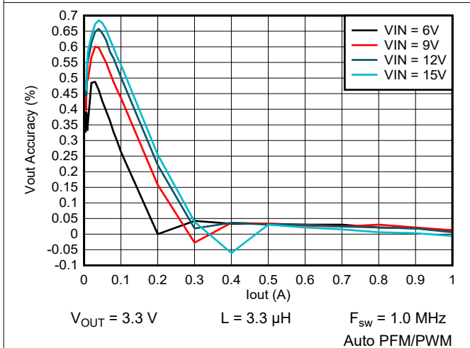
Figure 9-24. Output Voltage vs Output Current
