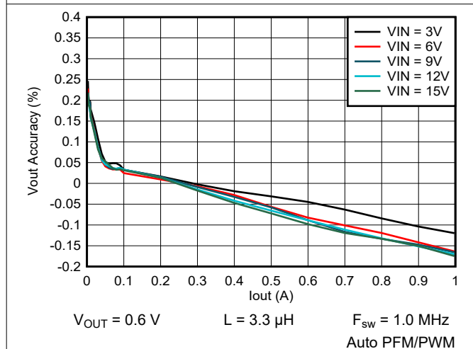
Figure 9-60. Output Voltage vs Output Current
