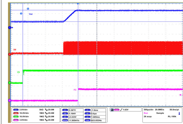
Figure 9-62. Start-Up Timing
