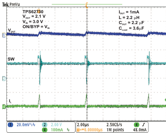
Figure 17. DC/DC Mode Operation I_{OUT} = 1\text{ mA}
