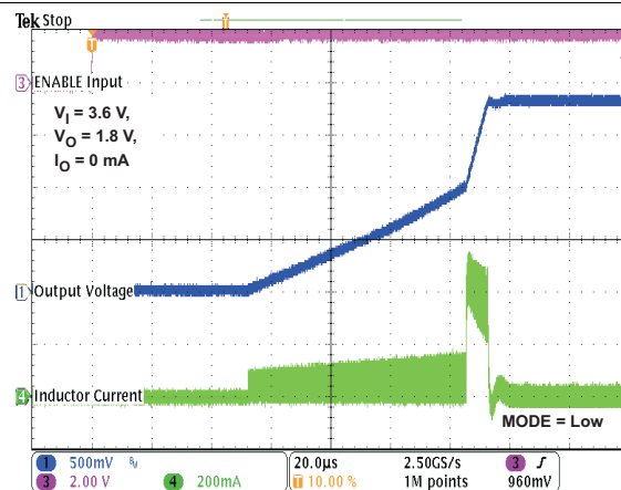
Figure 46. Start-Up
