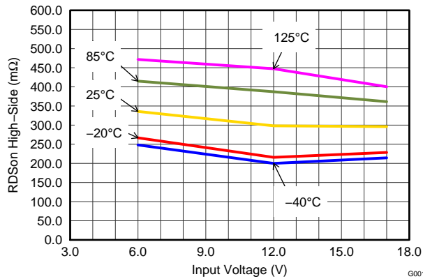
Figure 19. High-Side Switch
