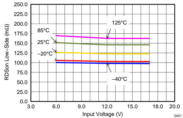
Figure 20. Low-Side Switch
