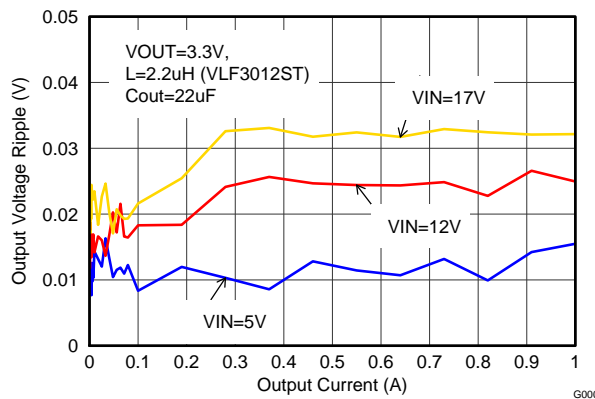
Figure 21. Output Voltage Ripple
