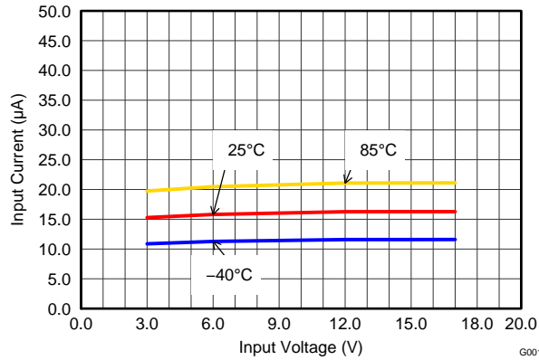
Figure 17. Quiescent Current
