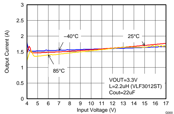
Figure 22. Maximum Output Current
