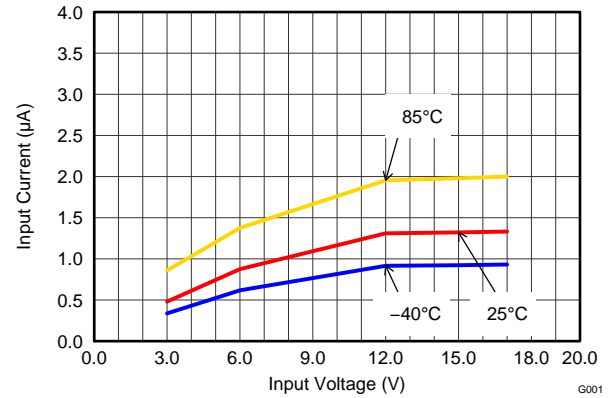
Figure 18. Shutdown Current
