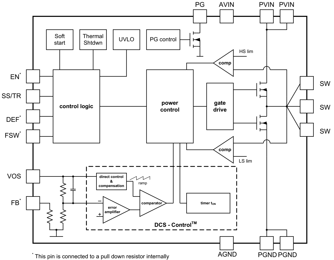
Figure 3. TPS62141/2/3 (Fixed Output Voltage)
