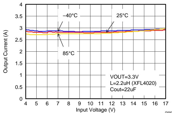
Figure 26. Maximum Output Current
