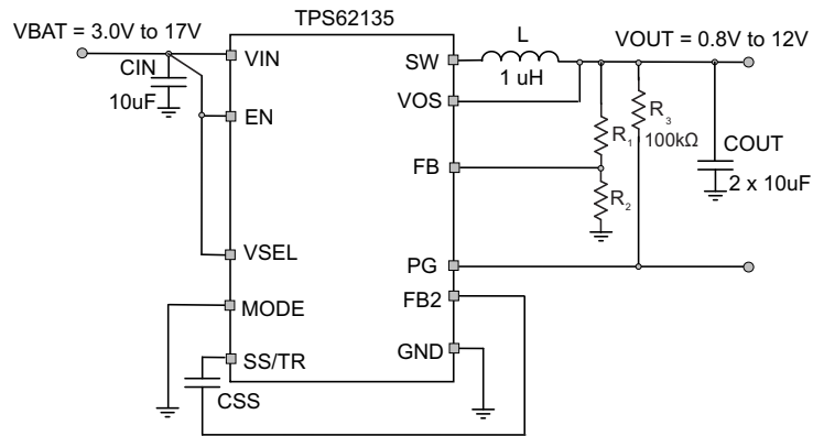
Figure 79. Connecting CSS to the Internal Analog Ground by using FB2
