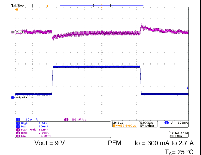
Figure 59. Load Transient Response
