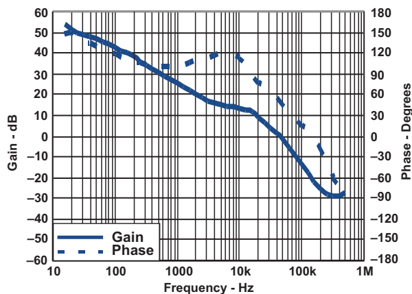
CLOSED LOOP RESPONSE, VIN (5 V), 4 A
