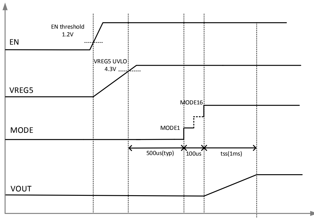
Figure 20. Power-Up Sequence
