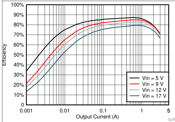
Figure 9. V_{OUT} = 0.95\text{ V} Efficiency, L = 1.2\text{ }\mu\text{H}
