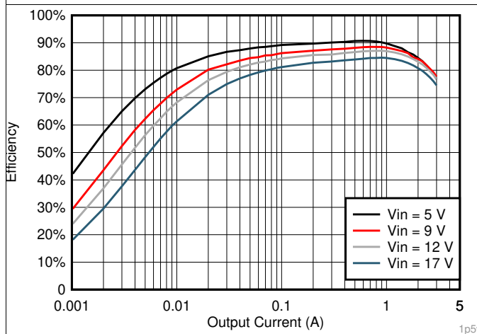
Figure 11. V_{OUT} = 1.5\text{ V} Efficiency, L = 1.5\text{ }\mu\text{H}
