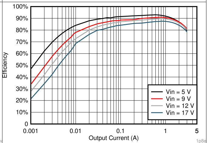
Figure 12. V_{OUT} = 1.8\text{ V} Efficiency, L = 2.2\text{ }\mu\text{H}
