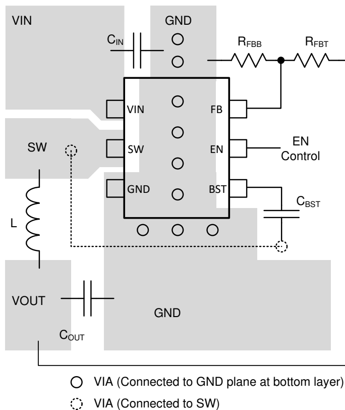
Figure 28. TPS563202 Layout
