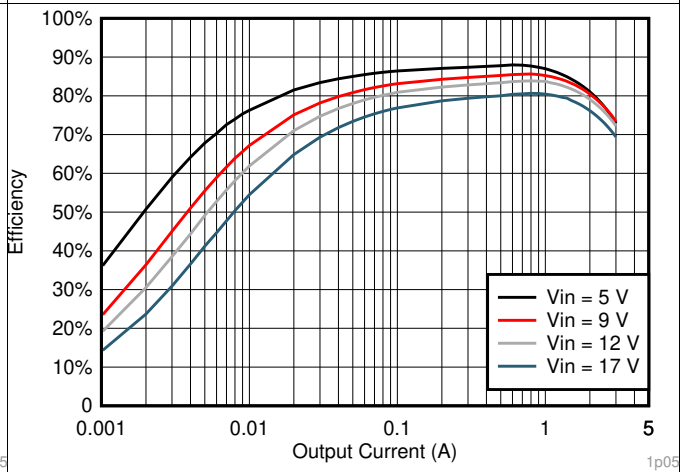
Figure 10. V_{OUT} = 1.05\text{ V} Efficiency, L = 1.2\text{ }\mu\text{H}
