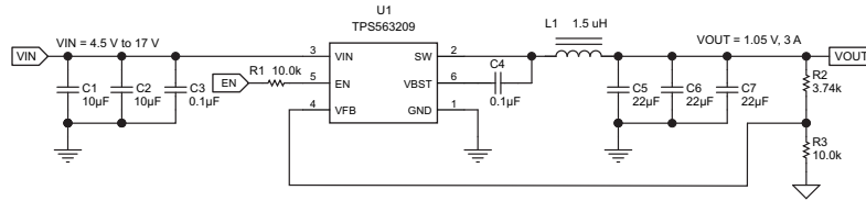
Figure 33. TPS563209 1.05V/3A Reference Design
