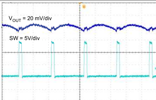
Figure 26. TPS562201 Output Voltage Ripple, I_{OUT} = 0.25 \text{ A}
