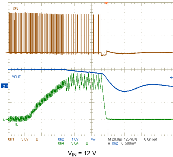
Figure 8-20. Overcurrent Protection – Overload
