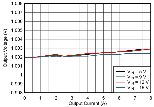
Figure 8-5. Load Regulation
