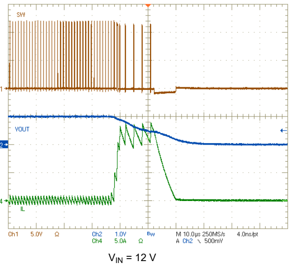
Figure 8-21. Overcurrent Protection – Short
