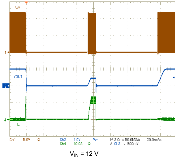
Figure 8-22. Overcurrent Protection – Hiccup and Recover
