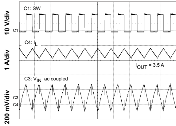
Figure 42. Input Ripple CCM
