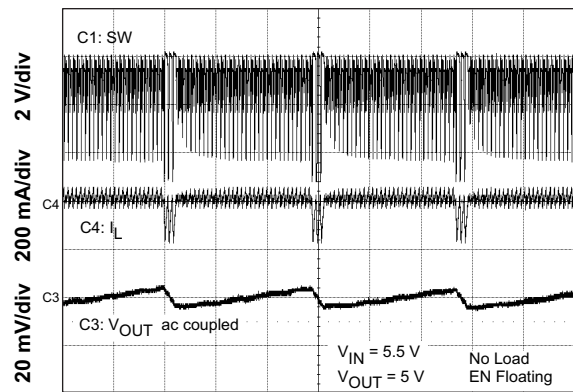
Figure 44. Low Dropout Operation
