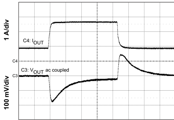
Figure 35. Load Transient
