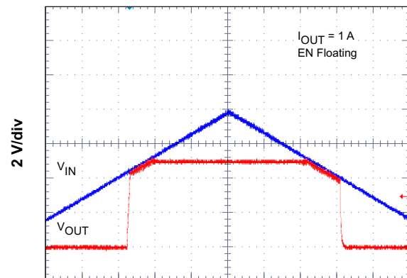
Figure 46. Low Dropout Operation
