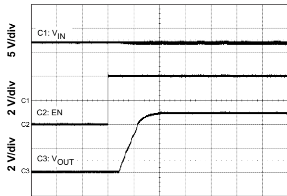
Figure 38. Startup With EN
