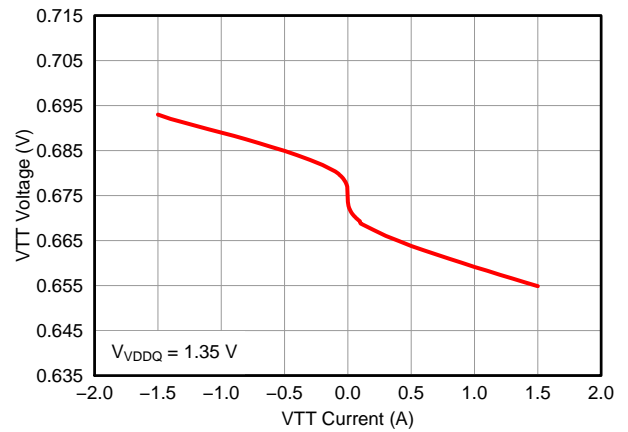
Figure 22. VTT Load Regulation
