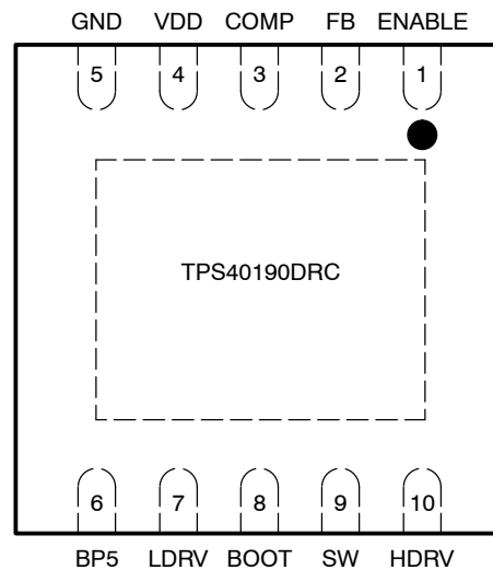
DRC PACKAGE (TOP VIEW)
