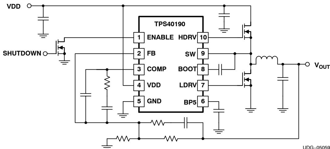
SIMPLIFIED APPLICATION DIAGRAM
