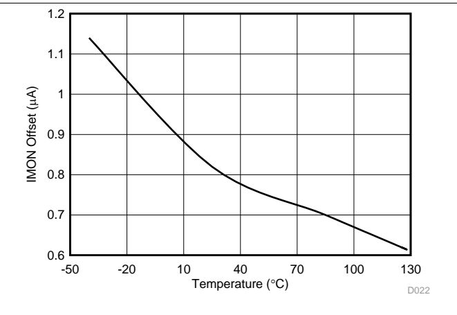
Figure 24. IMON Offset vs Temperature
