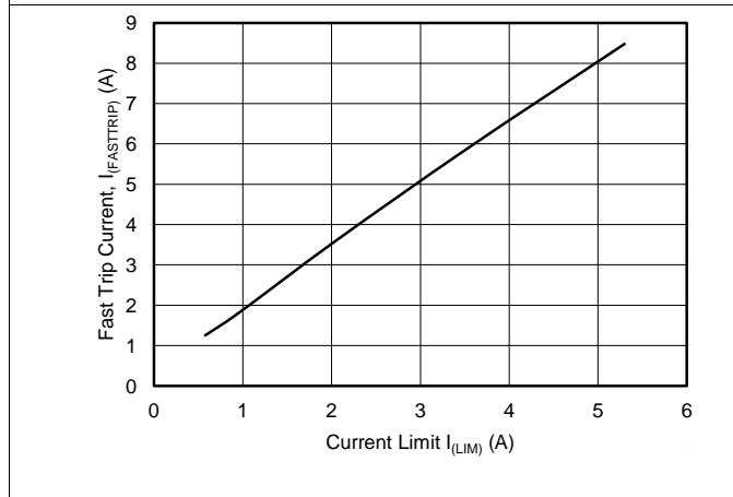
Figure 23. Fast Trip Threshold vs Current Limit
