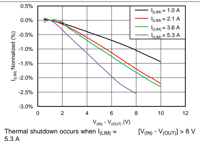
Figure 20. Current Limit Normalized (%) vs V_{(IN)} - V_{(OUT)}
