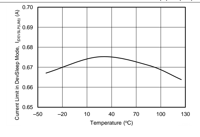
Figure 22. Current Limit in DevSleep Mode vs Temperature
