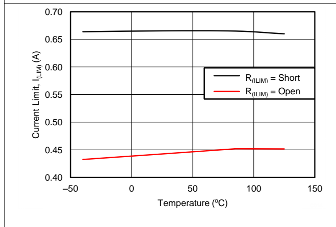
Figure 21. Current Limit for R_{(ILIM)} = \text{Open and Short vs Temperature}
