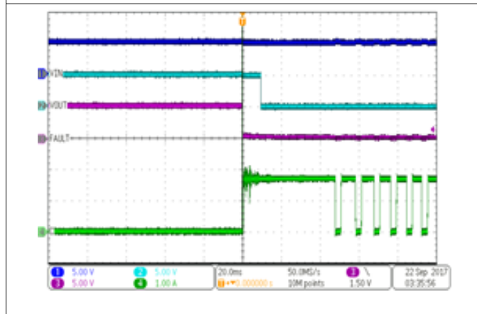
Figure 17. Screw Driver Short on VBUS
