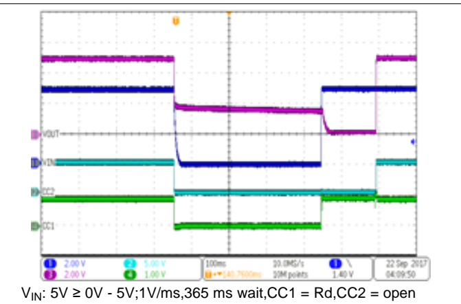
Figure 18. Brownout Test
