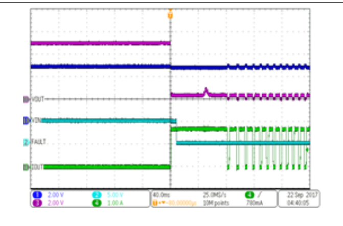
Figure 16. Extended Period OUT Short Event
