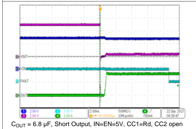
Figure 15. Out Short Event
