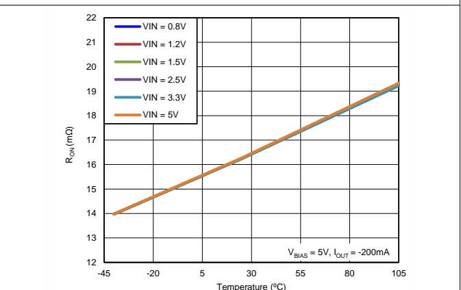
Figure 6. R_{ON} vs. Temperature ( V_{BIAS} = 5 V, Single Channel)
