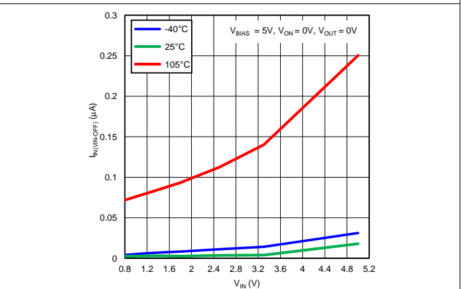
Figure 4. Off-State V_{IN} Current vs. V_{IN} (Single Channel)
