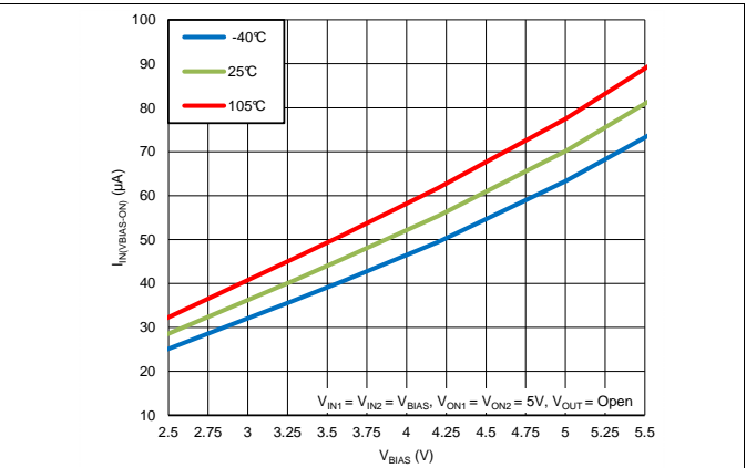
Figure 2. Quiescent Current vs. V_{BIAS} (Single Channel)
