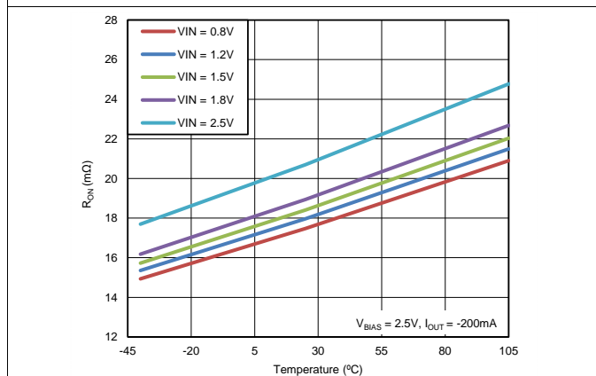
Figure 5. R_{ON} vs. Temperature ( V_{BIAS} = 2.5 V, Single Channel)
