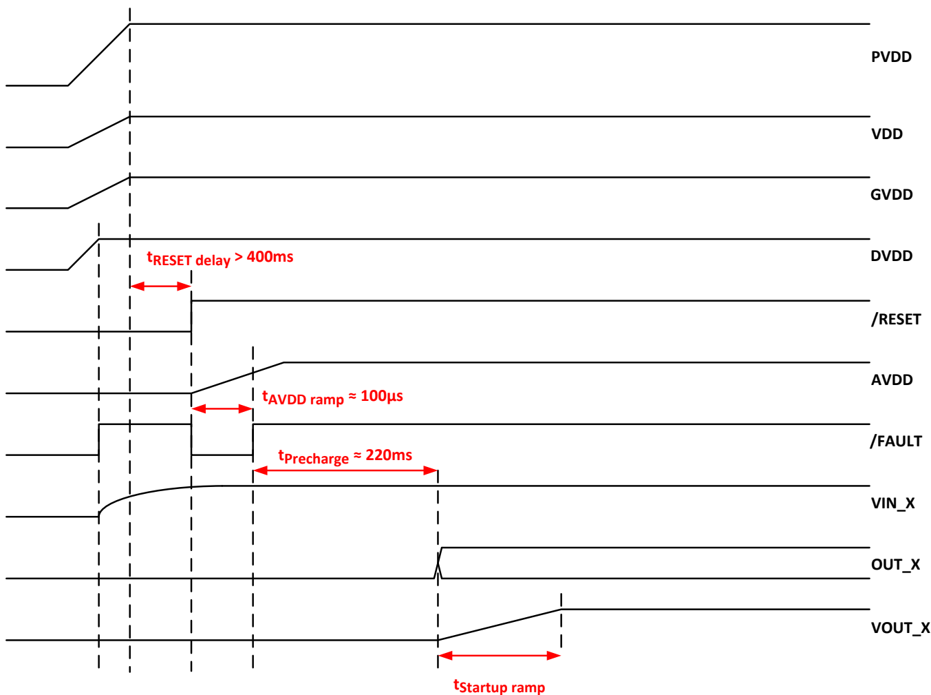
Figure 7. Startup Timing
