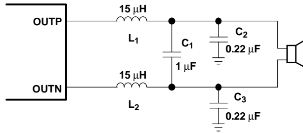
Figure 16. Typical LC Output Filter, Cutoff Frequency of 41 kHz, Speaker Impedance = 4Ω
