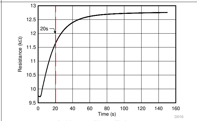
Figure 10. Thermal Response Time
