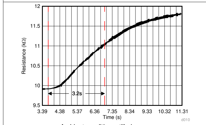
Figure 9. Step Response
