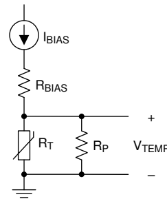
Figure 16. Current Biasing Circuit With Linear Thermistor
