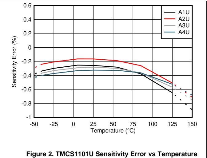
Figure 2. TMCS1101U Sensitivity Error vs Temperature
