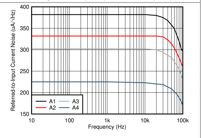
Figure 12. Input-Referred Noise vs Frequency
