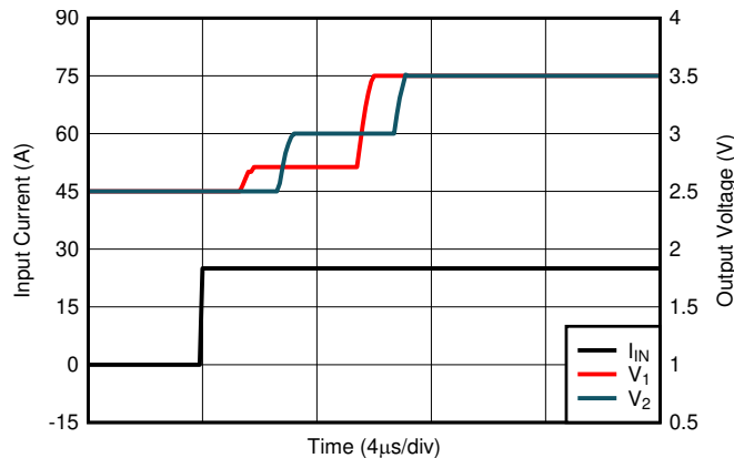
Figure 42. Transient Response to Input-Current Step Sufficient for 1-V Output Swing
