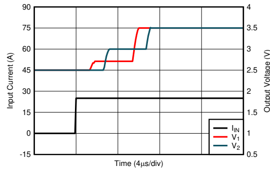
Figure 22. Transient Step Response
