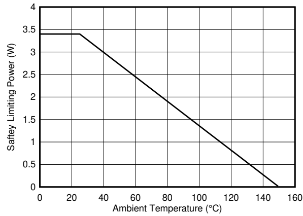
Figure 20. Thermal Derating Curve for Safety-Limiting Power
