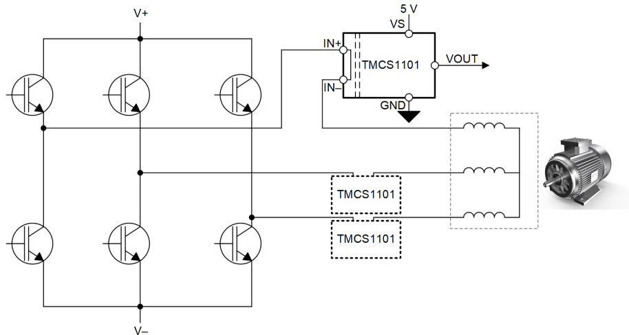
Figure 46. Inline Motor Phase Current Sensing
