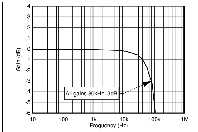
Figure 7. Sensitivity vs Frequency, All Gains Normalized to 1 Hz
