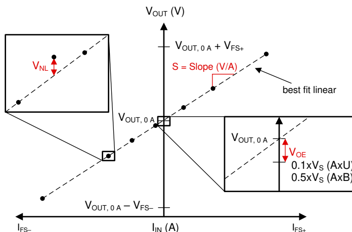
Figure 21. Sensitivity, Offset, and Nonlinearity Error
