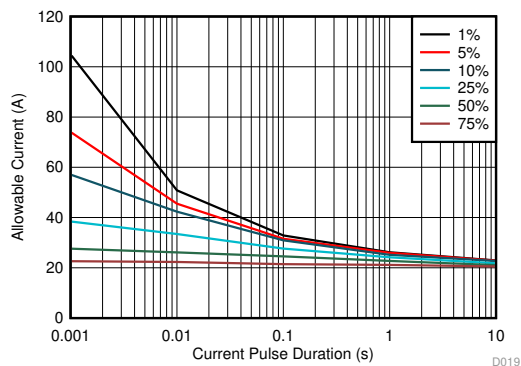
Figure 27. Maximum Repetitive Pulsed Current vs Pulse Duration
