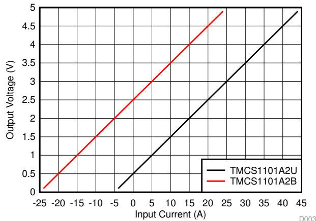
Figure 44. Output Voltage Relationship to Input Current for TMCS1101A2B and TMCS1101A2U
