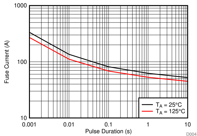
Figure 30. Single-Pulse Leadframe Capability
