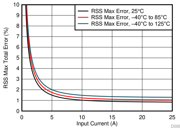
Figure 45. RSS Error vs Input Current
