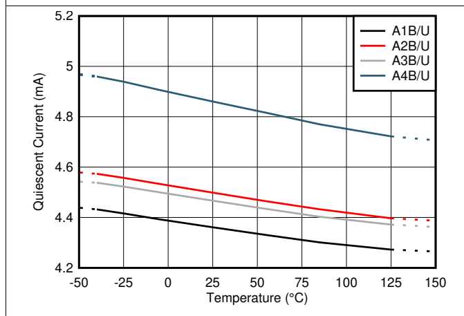
Figure 11. Quiescent Current vs Temperature
