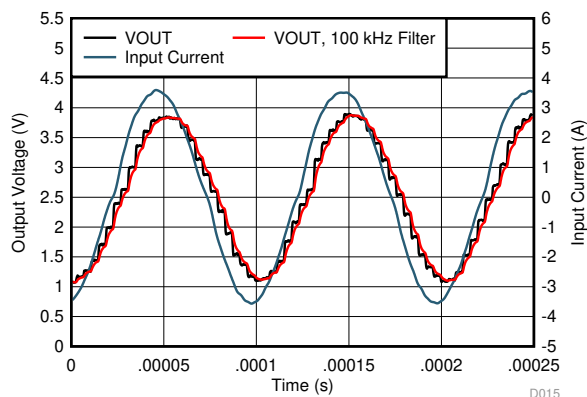
Figure 41. Response Behavior to 10kHz Sine Wave Input Current
