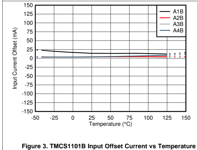
Figure 3. TMCS1101B Input Offset Current vs Temperature
