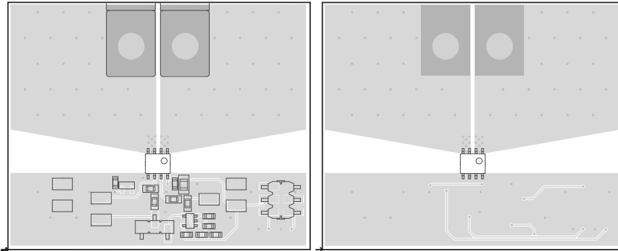
Figure 50. Recommended Board Top (Left) and Bottom (Right) Plane Layout
