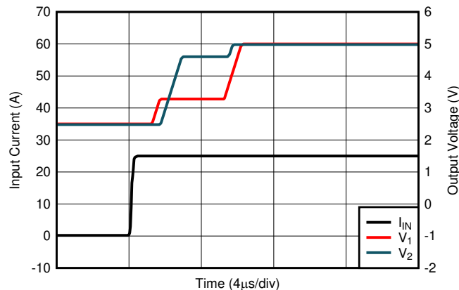
Figure 43. Transient Response to a Large Input Current Step
