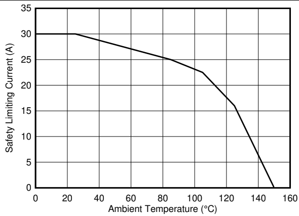
Figure 18. Thermal Derating Curve for Safety-Limiting Current, Side 1
