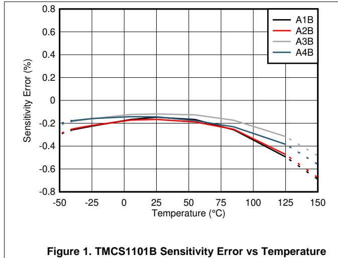
Figure 1. TMCS1101B Sensitivity Error vs Temperature
