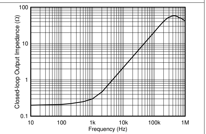
Figure 10. Output Impedance vs Frequency
