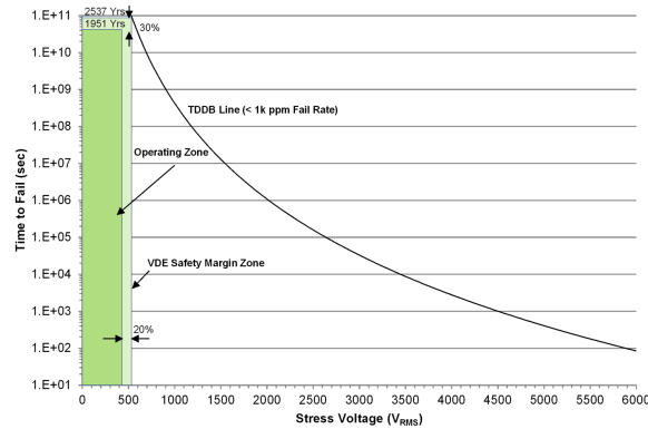
Figure 31. Insulation Lifetime
