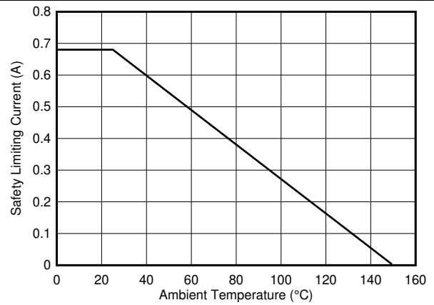
Figure 19. Thermal Derating Curve for Safety-Limiting Current, Side 2
