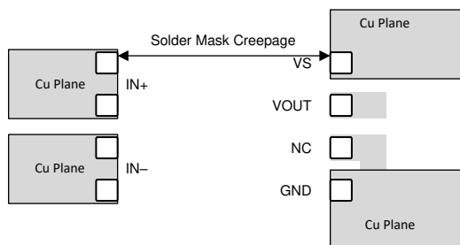
Figure 49. Layout for System Creepage Requirements
