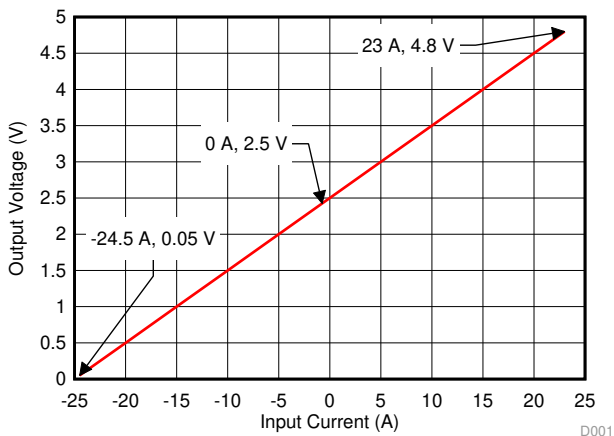
Figure 47. Application Example Design Transfer Curve
