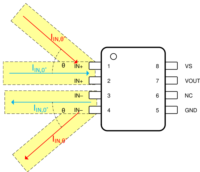
Figure 48. Magnetic Field Generated by Input Current Trace
