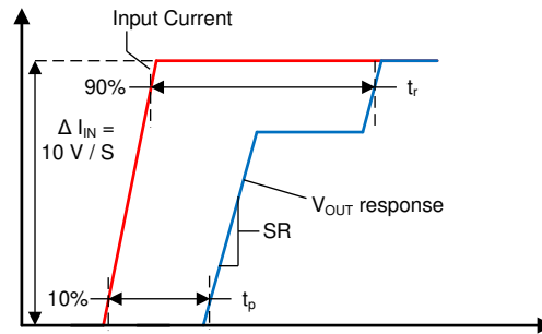
Figure 24. Current Overload Transient Response
