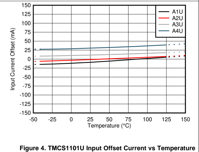
Figure 4. TMCS1101U Input Offset Current vs Temperature
