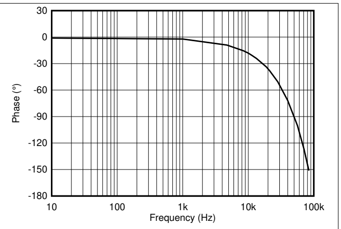
Figure 8. Phase vs Frequency, All Gains
