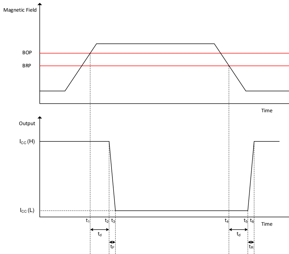
Figure 8-8. Propagation Delay
