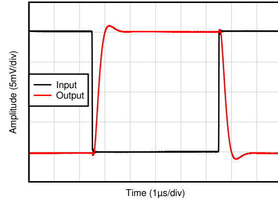
C_L = 20\text{ pF} , G = -1 , 20-mV step response C011
