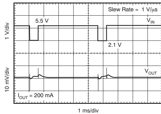
Figure 20. TLV70018 Line Transient Response
