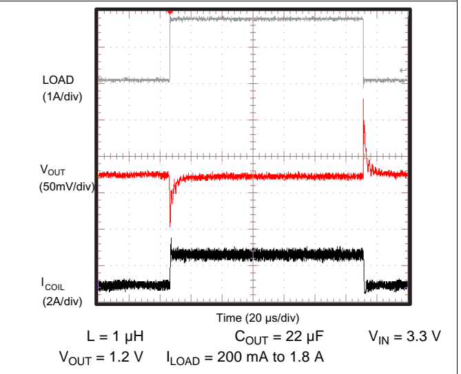
Figure 14. Load Transient
