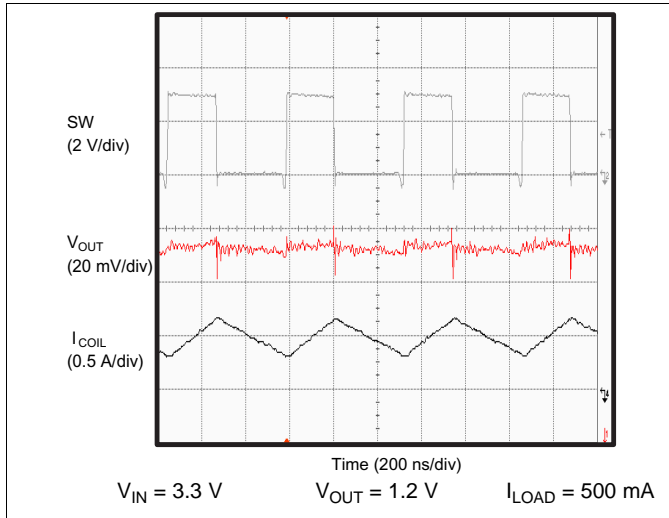
Figure 11. Typical Application (PWM Mode)
