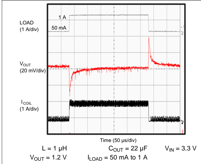
Figure 13. Load Transient
