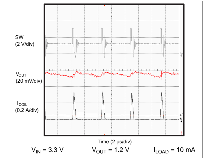
Figure 12. Typical Application (PFM Mode)
