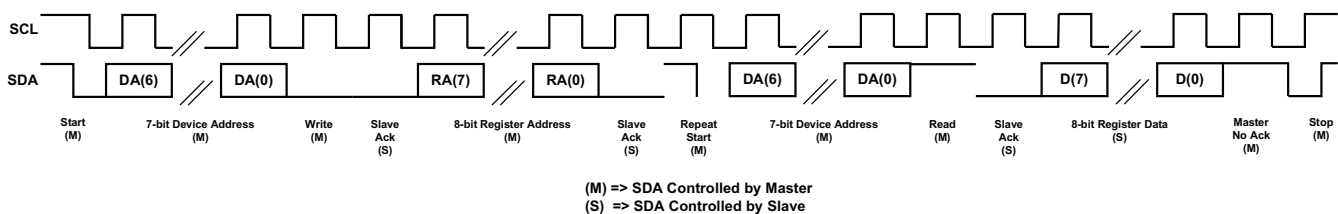
Figure 17. I2C Read
