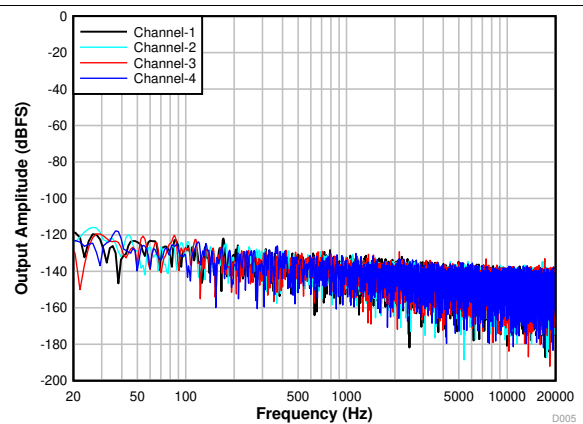
Figure 14. FFT With Idle Input
