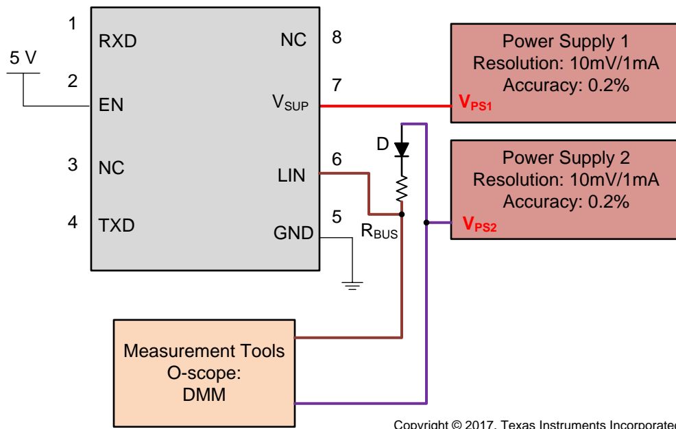
Figure 12. V_{SUP\_NON\_OP} Param 1154/56
