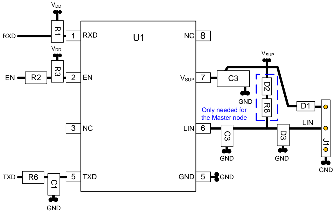
Figure 33. Layout Example
