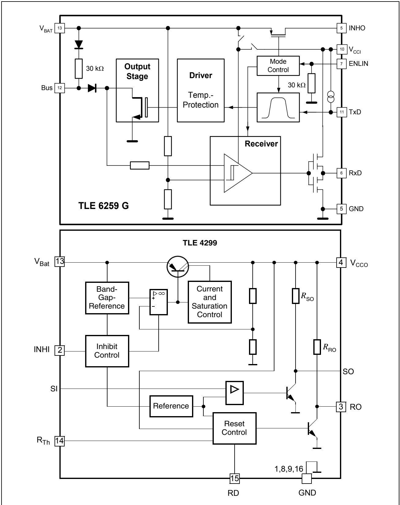
Figure 2 Block Diagram
