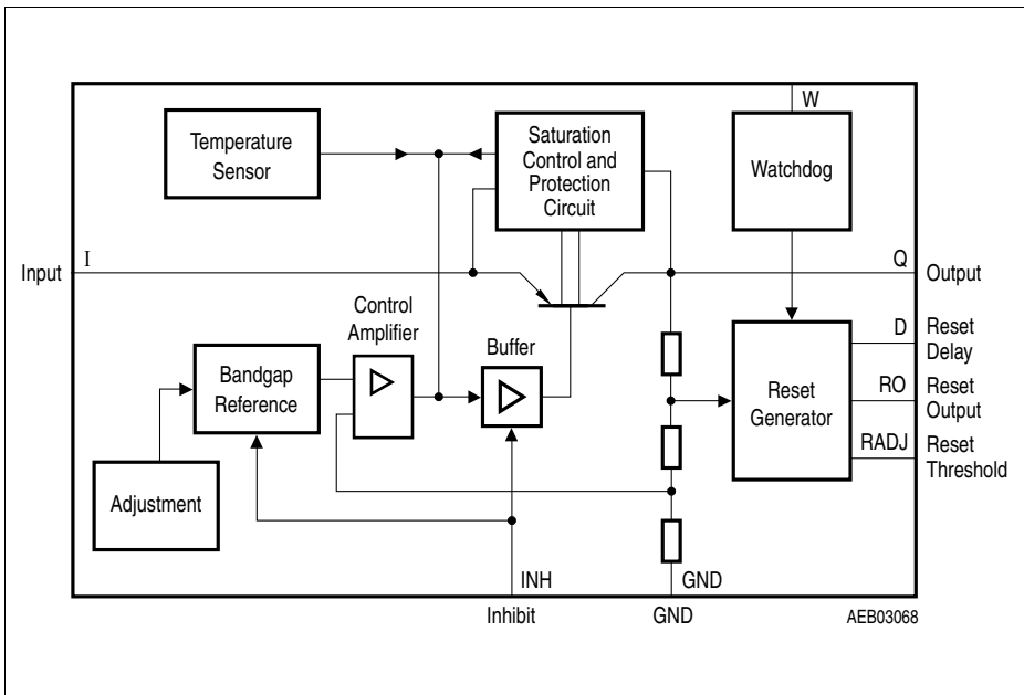
Figure 2 Block Diagram
