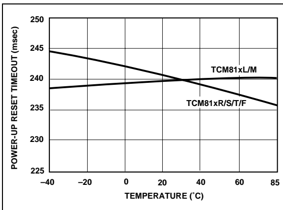
FIGURE 3-3: Power-Up Reset Timeout vs. Temperature.
