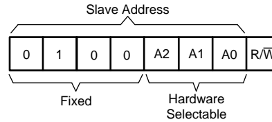
Figure 26. TCA9534 Address
