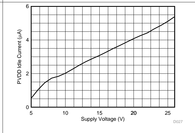
Figure 22. PVDD Standby Current vs Voltage
