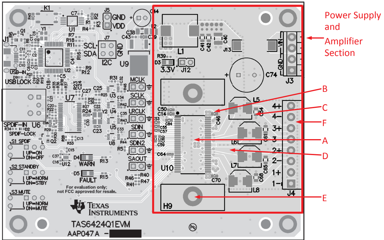
Figure 85. EVM Layout
