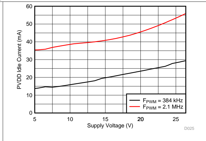
Figure 20. PVDD Current vs Voltage
