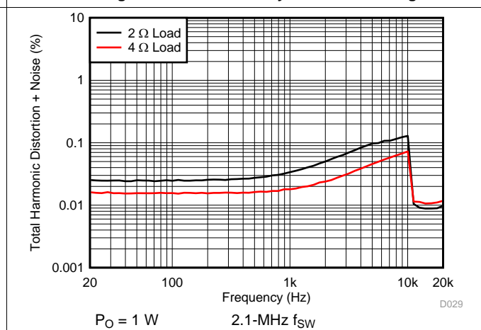
Figure 24. PBTL THD+N vs Frequency
